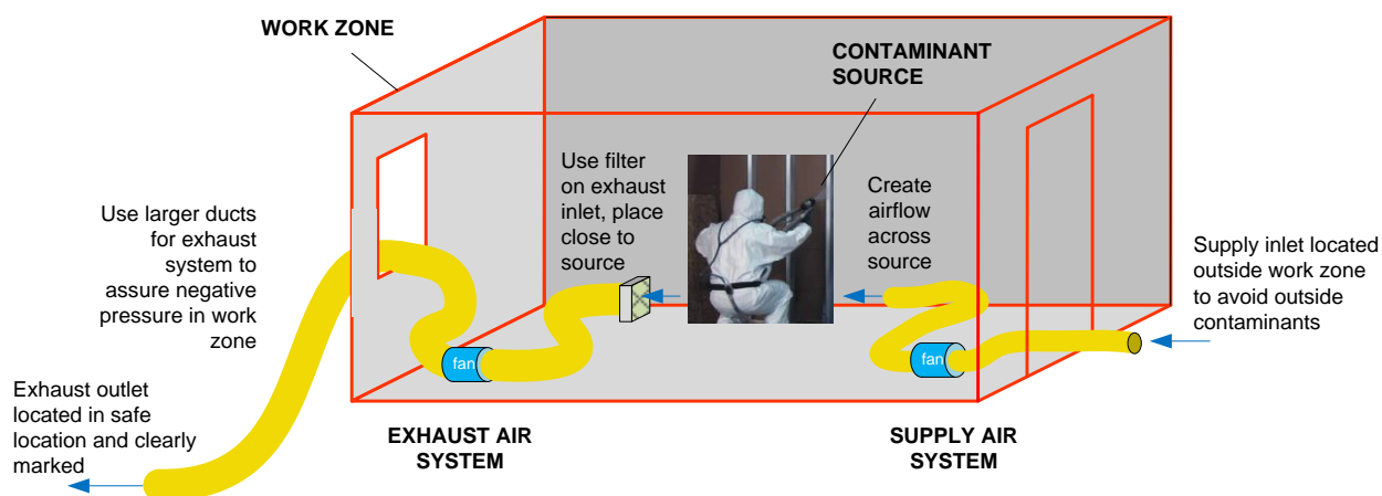
FIGURE 4 - Example of a Two-Fan Ventilation System (active exhaust and supply systems) for Interior SPF Application.
